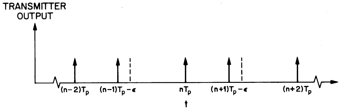
Fig. 2. Two-pulse staggered sampling pattern.
