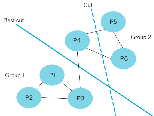
FIGURE 4. Spectral clustering of a graph relies on recursive binary partitions, or “cuts,” of the graph. At a given stage, the algorithm chooses among all possible cuts (as illustrated by the dotted line) the “best” cut (shown by the solid line) that maximizes within-community connections and minimizes between-community connections of the resulting subgraphs.
