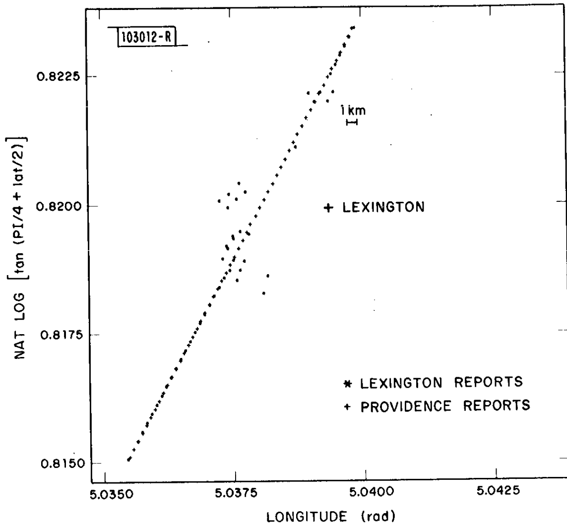
Fig. 10. Expanded view of portion of aircraft code 3502 tracks.
