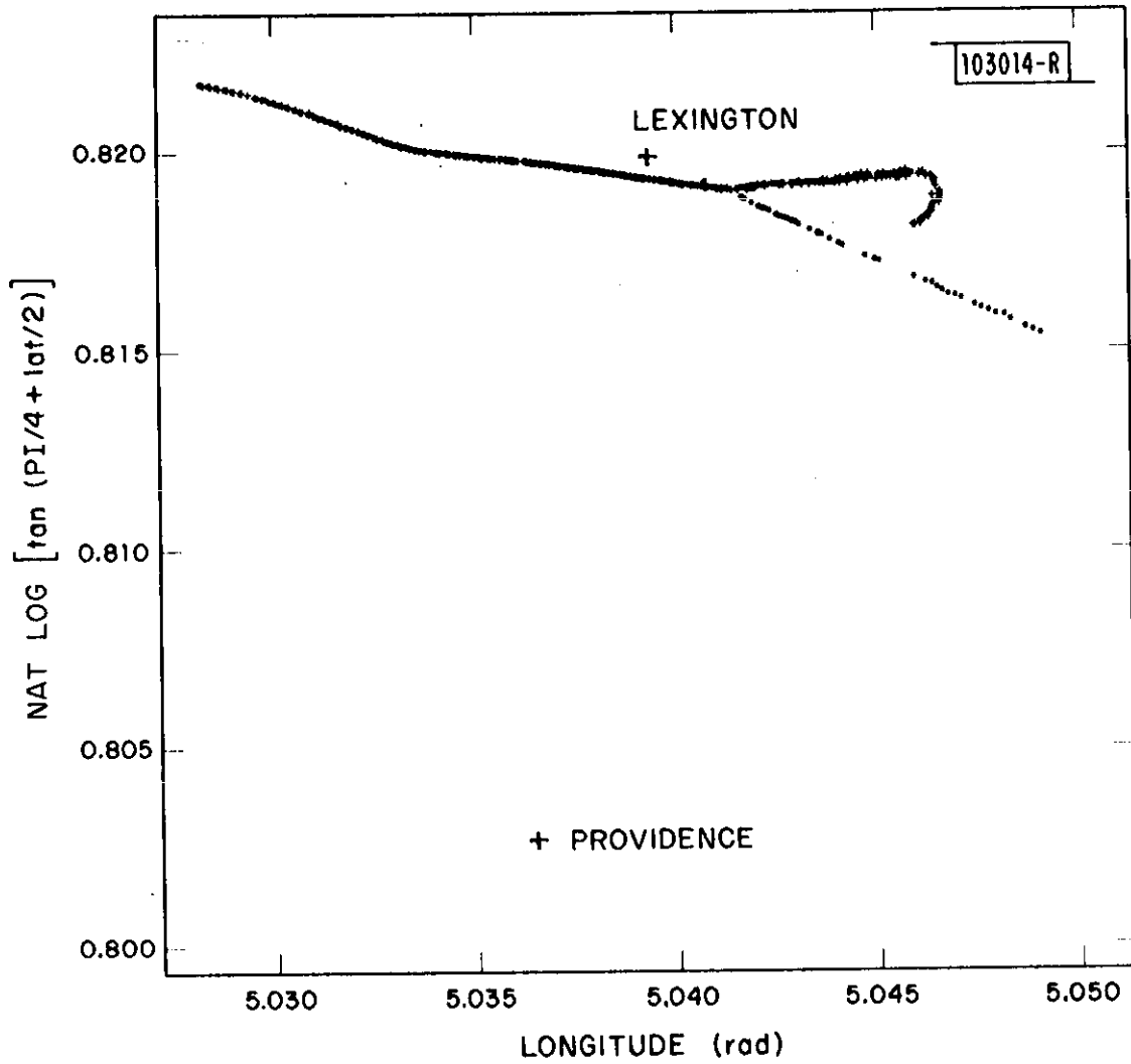
Fig. 12. Aircraft code 2417 after bias removal.
