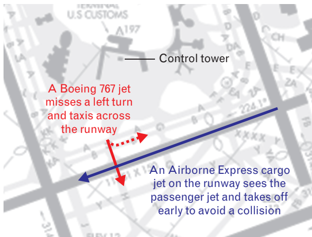
FIGURE 2. A representative runway incursion at New York’s JFK International Airport. On 6 July 2005, an Israir Boeing 767 taxied across an active runway instead of turning to follow the taxiway (dashed line), and blundered directly in front of an Airborne Express DC-8 that was taking off. The Airborne Express aircraft lifted off early and cleared the Boeing 767 by less than a hundred feet. Poor visibility in rain and fog prevented either aircraft from being visible from the air traffic control tower. (JFK airport graphic courtesy of the FAA.)
