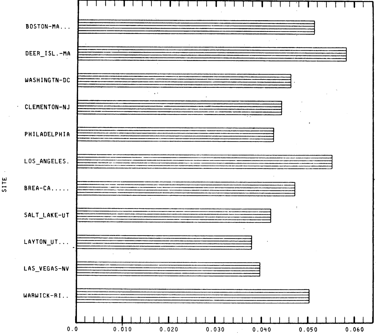
Fig. IV-12. Azimuth error (standard deviation in degrees).
