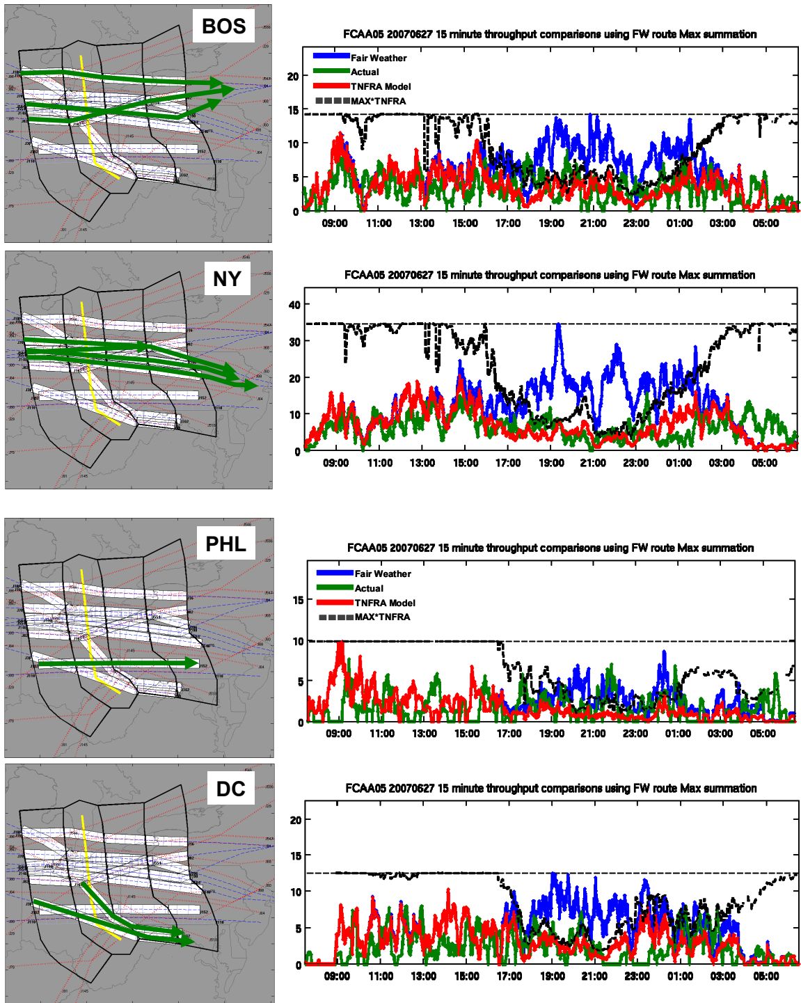
Figure 3-7. Tactical FCAA05 AFP throughput assessment, with route availability and usage (estimated vs. actual) deconstructed for individual traffic flows to Boston, metro-NY (EWR, LGA, and JFK), Philadelphia, and metro-DC (IAD, DCA, and BWI) airports. Throughput time series results (right-side) are presented as in Figure 3-6.
