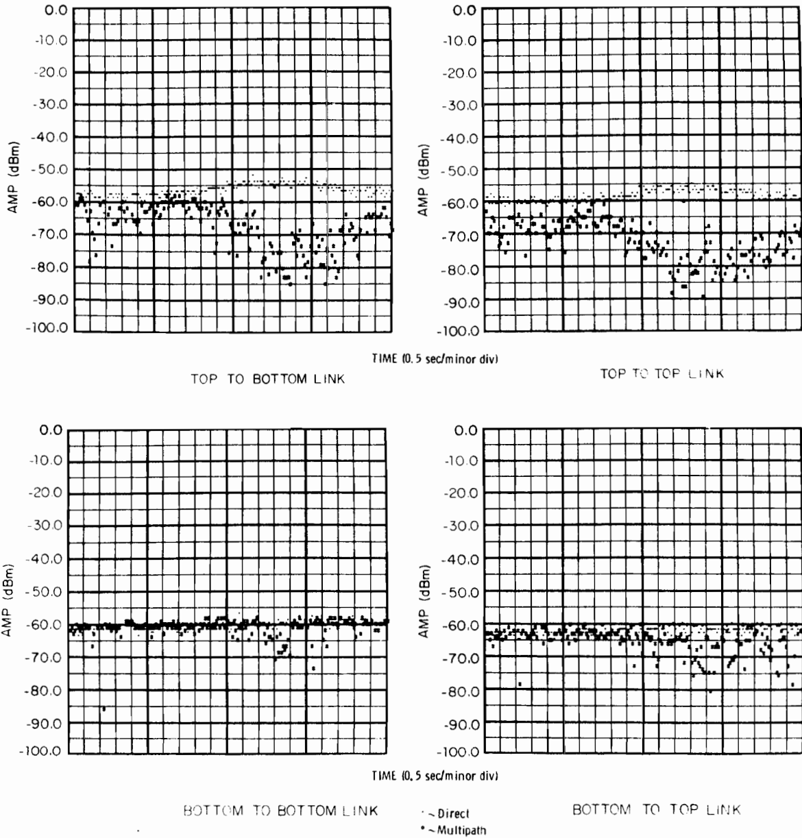
Fig. 5.20. Frozen Lake (Low Grazing Angle) Multipath Instantaneous Signal Strength.
