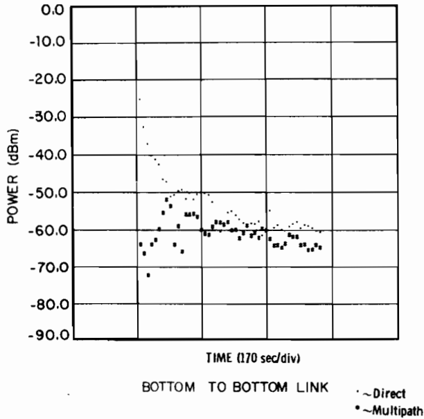
Fig. 5.22. Frozen Lake (High Altitude) Multipath Average Signal Strength.
