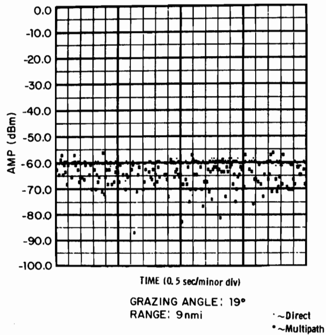
Fig. 5.4. Ocean (Sea State 1) Multipath Instantaneous Signal Strength.
