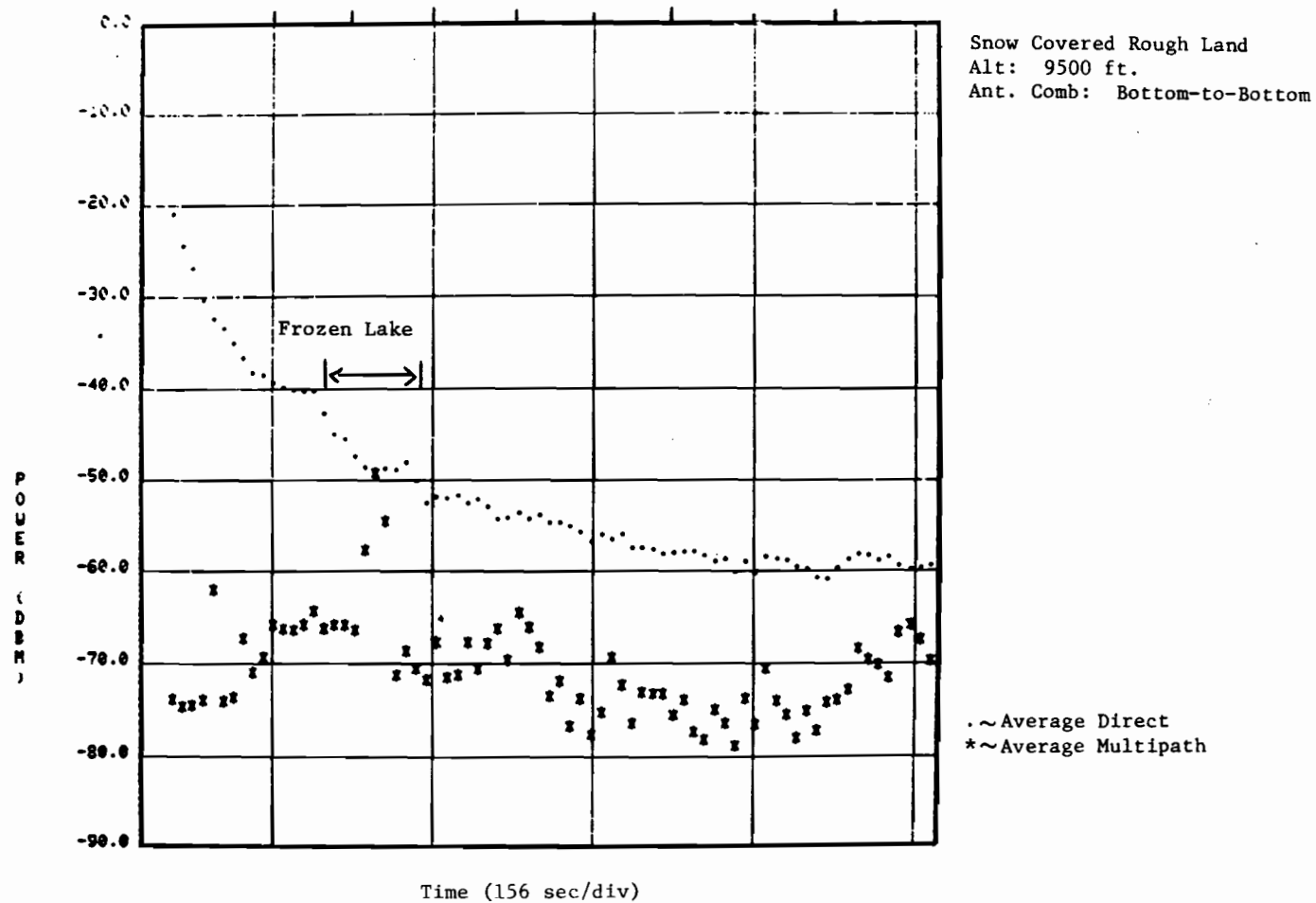
Fig. 5.37. Snow Covered Rough Land Multipath Average Signal Strength.
