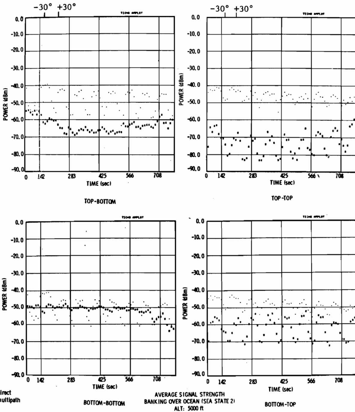
Fig. 5.39. Multipath Sensitivity to Banking.
