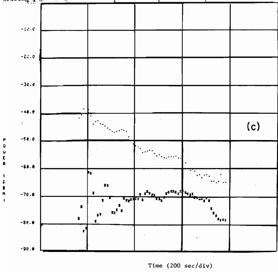
Fig. 5.7(c). Ocean (Sea State 1) Multipath Average Signal Strength.
