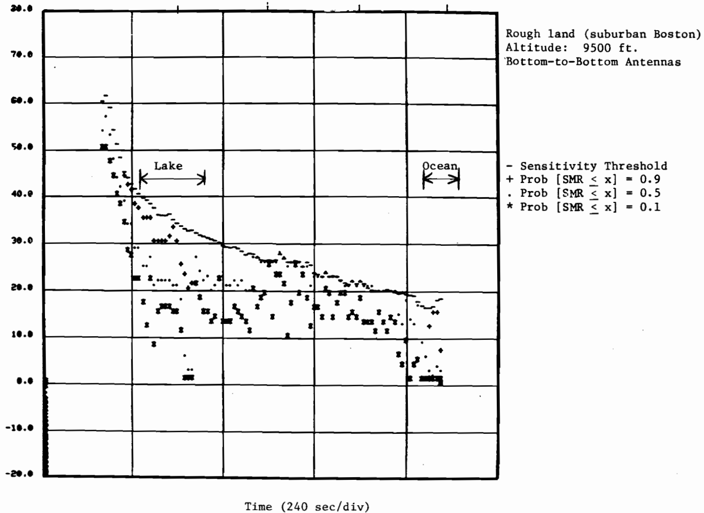
Fig. 5.35. Signal-to-Multipath Ratio Distribution Variation (Rough Land).
