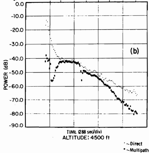
Fig. 5.7(a-b). Ocean (Sea State 1) Multipath Average Signal Strength.
