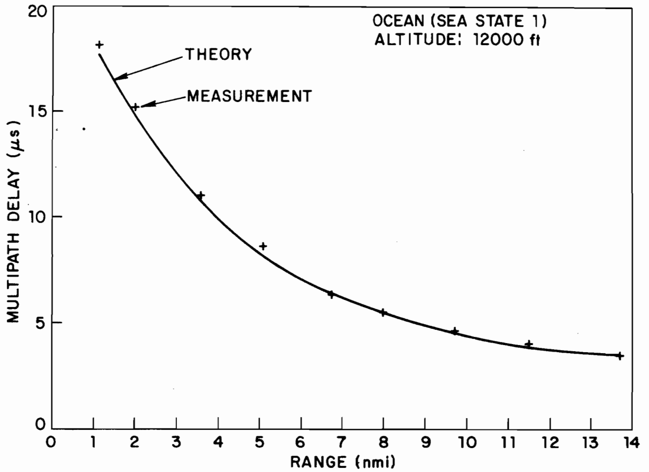
Fig. 5.3. Multipath Delay.
