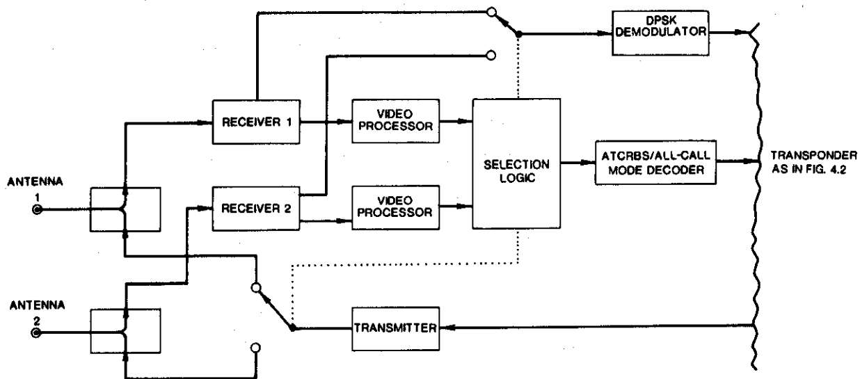
Fig. 4-3. Diversity Transponder.
