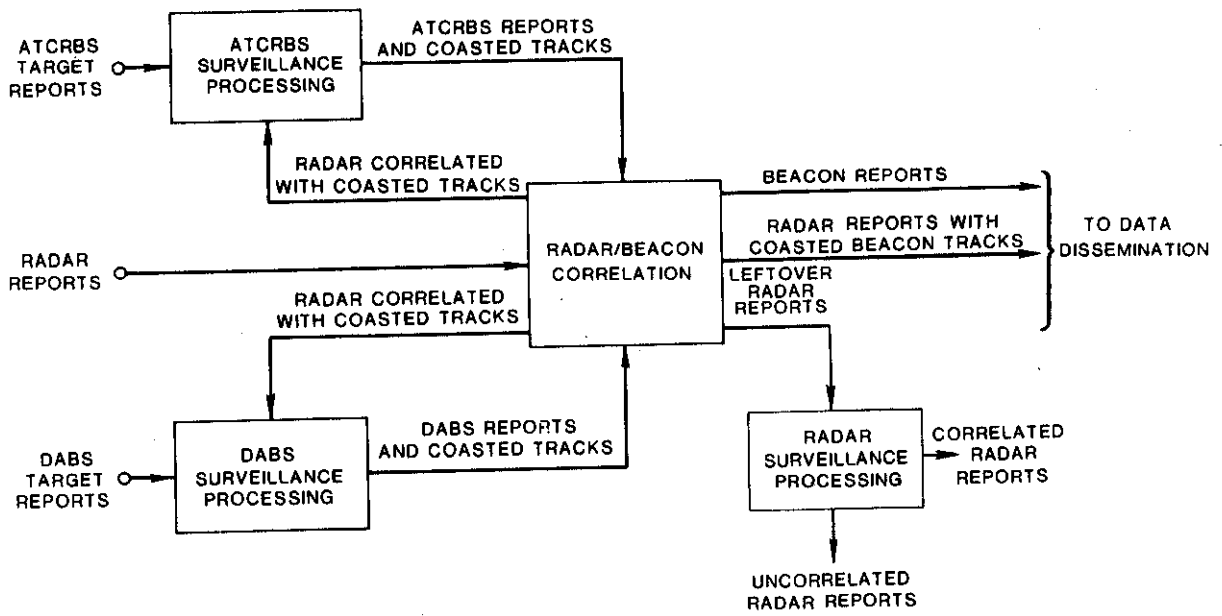
Fig. 3-14. Surveillance Processing.
