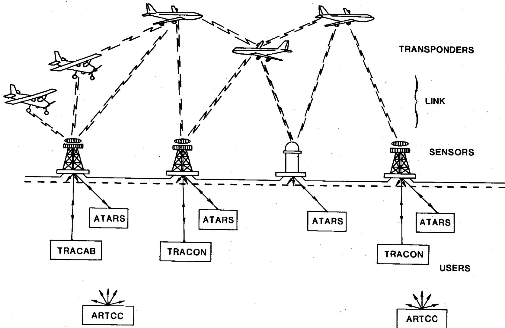
Fig. 1-1. DABS Elements.
