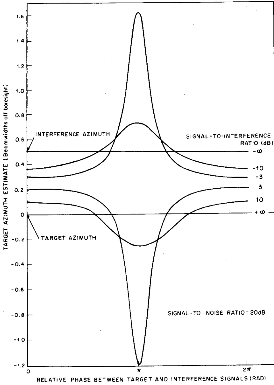
Fig. 5-6. Monopulse Estimate With Interference.
