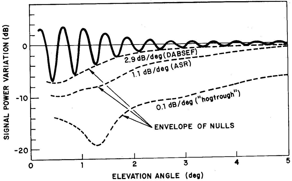
Fig. 5-1. Vertical Lobing.
