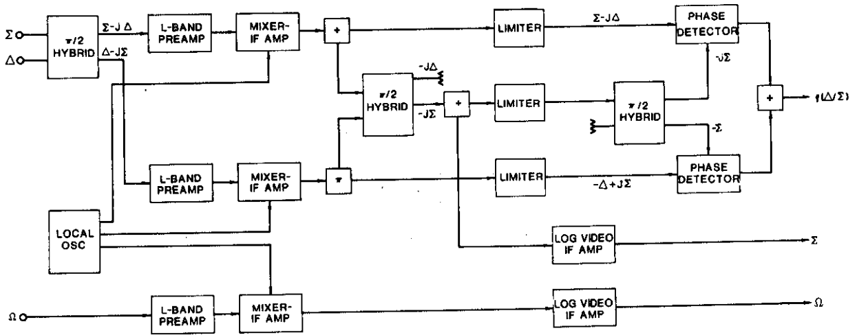
Fig. 3-10. Multi-channel Receiver.
