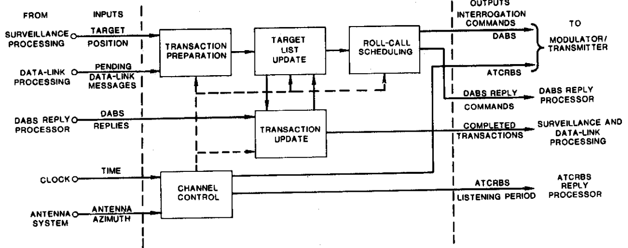
Fig. 3-5. Channel Management.
