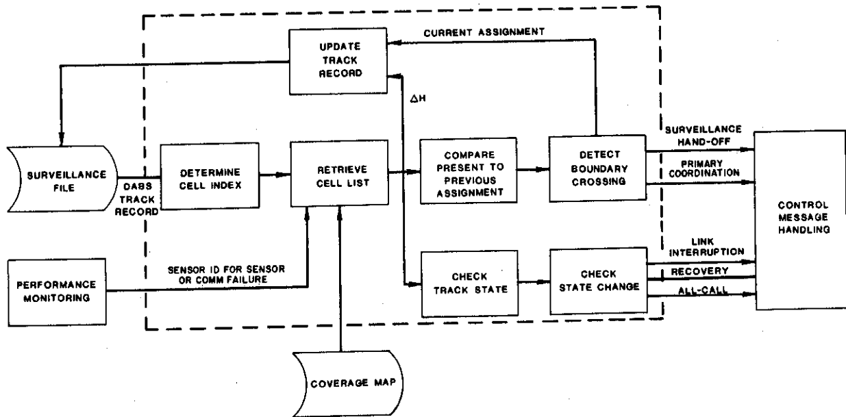
Fig. 3-23. Coverage Coordination.
