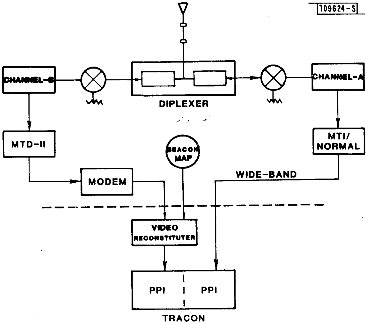
Fig. III-1. ASR-7 MTD/MTI at Burlington, VT Functional Block Diagram.
