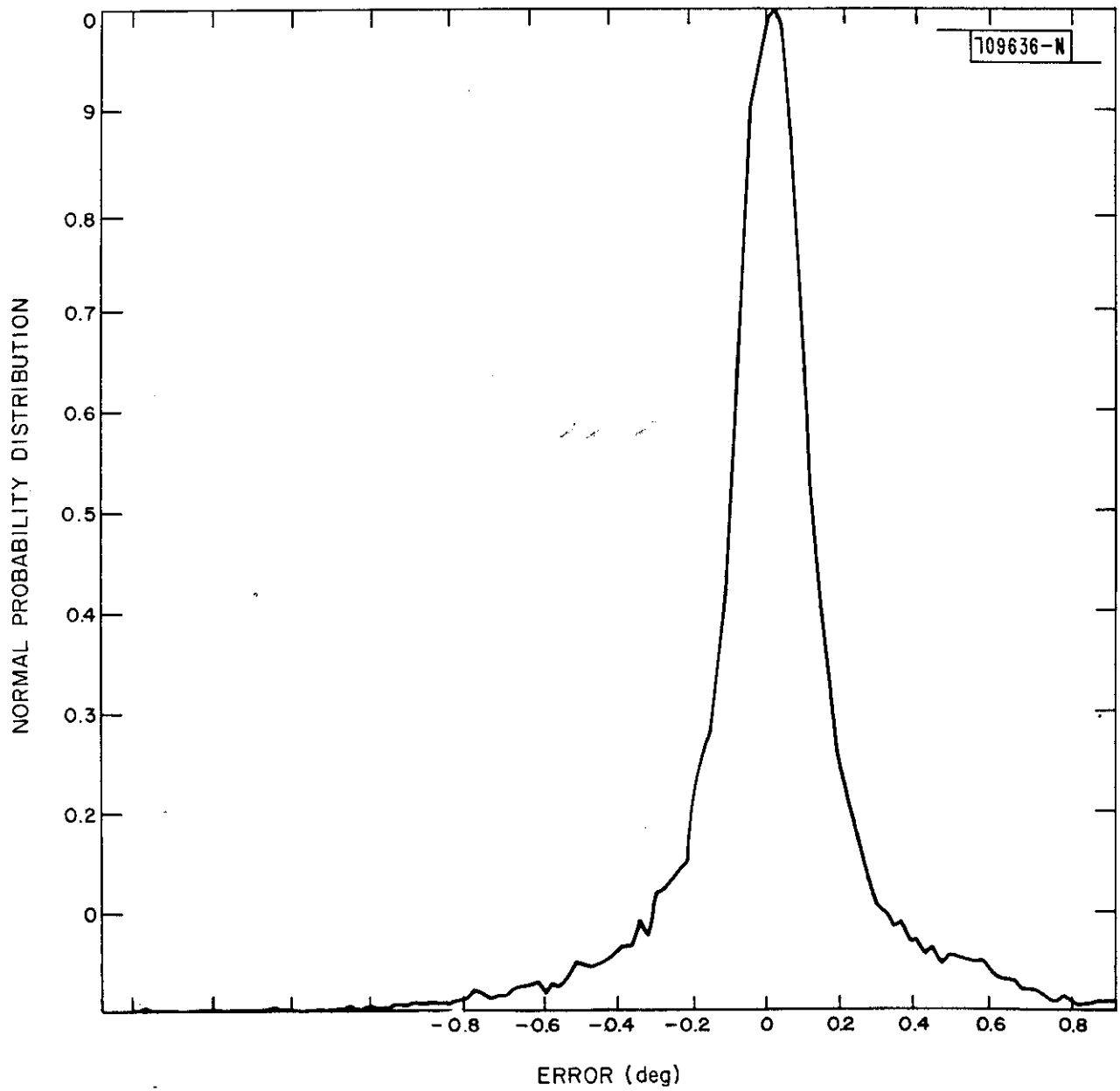
Fig. III-12. Total azimuth error distribution.
