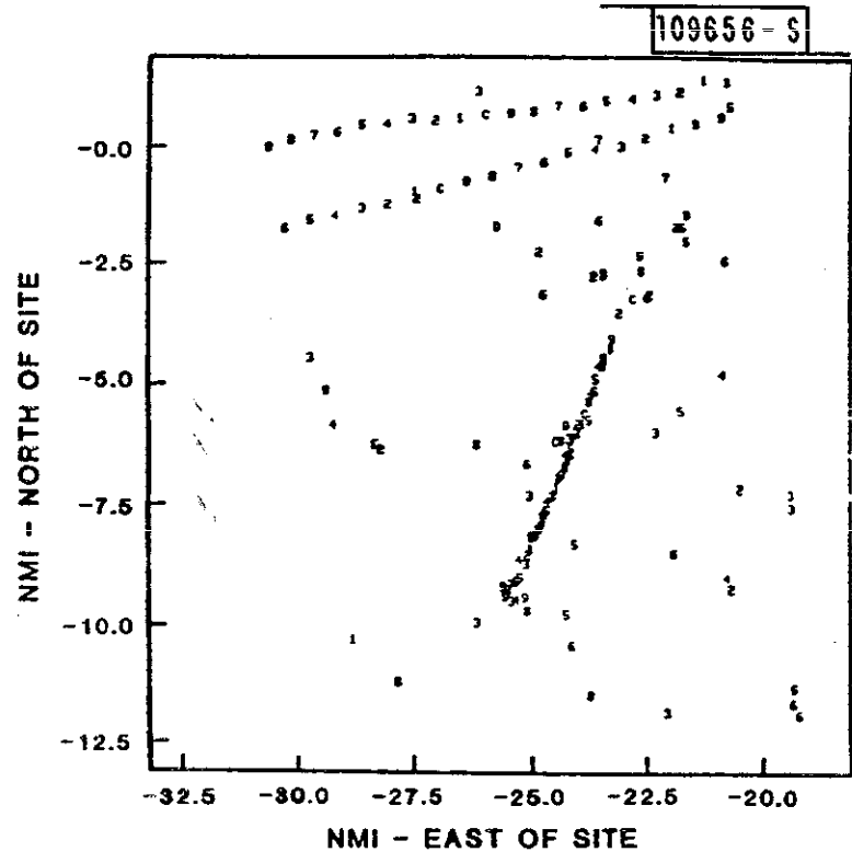
Fig. IV-9b. MTD target reports - linear CFAR.
