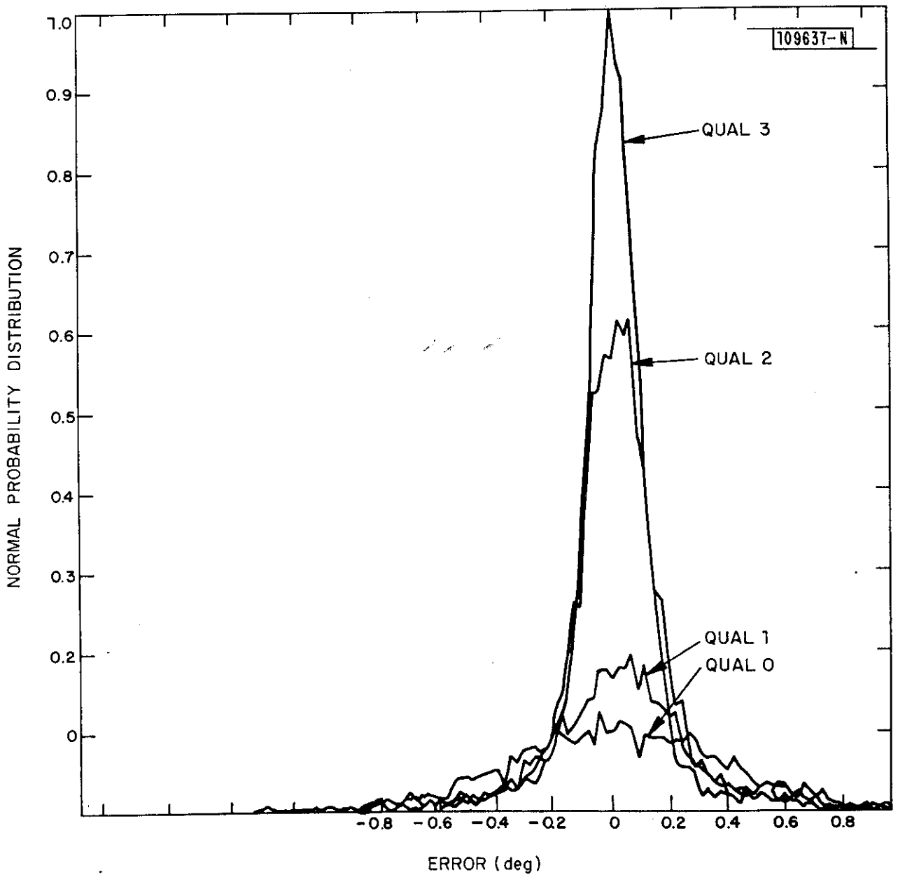
Fig. III-13. Azimuth error by target quality.
