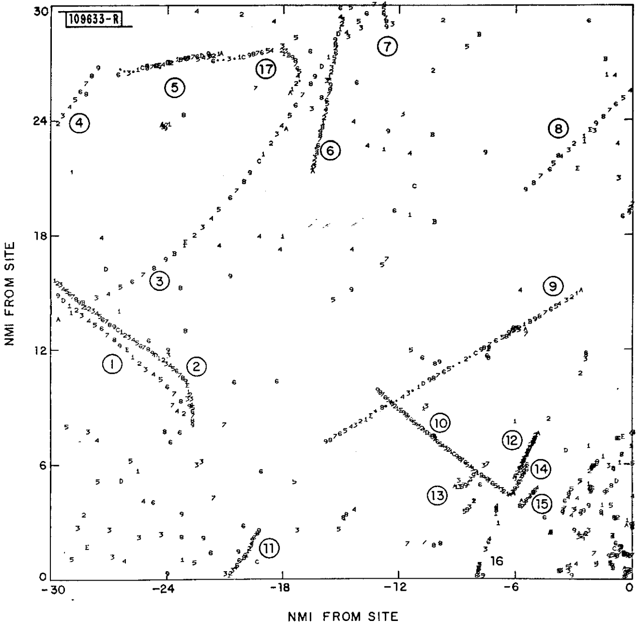
Fig. III-11a. MTD target reports (50 scans) at FAATC.
