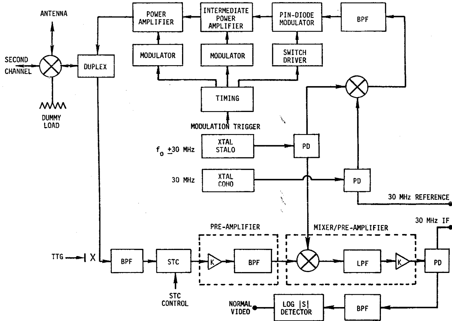
Figure 3.4.1-1 ASR-MTD Transmitter-Receiver Subsystem, Overall Block Diagram.
