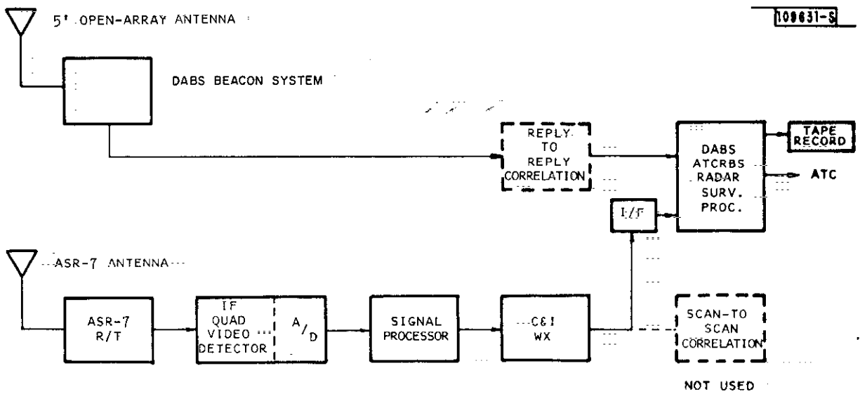
Fig. III-9. MTD/DABS at FAATC, functional block diagram.
