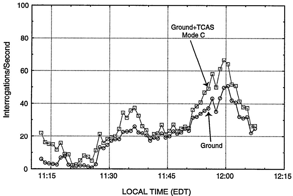
Figure 19. Measured interrogation rates, Lakeland, part A. As in Figure 12, the upper curve includes all ATCRBS interrogations while the lower curve includes all except TCAS Mode C interrogations. These observed rates are similar to interrogation rates measured in many locations [Reference 3].
