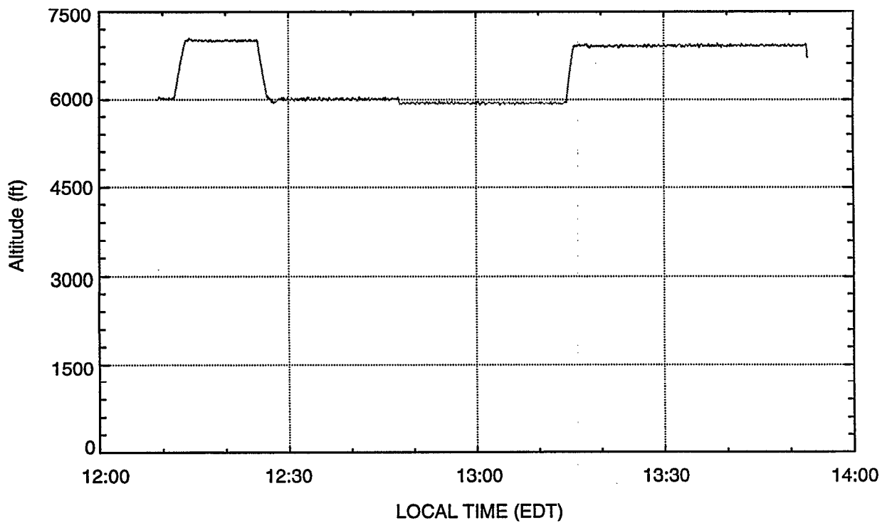
Figure 20. Flight path, Lakeland, part B. In the second segment, the AMF aircraft flew back across Florida, again passing over Orlando and Lakeland, and continuing on to Tampa. The flight continued by flying north and then southbound flying over Lakeland again. Reply rates were measured during this segment.
