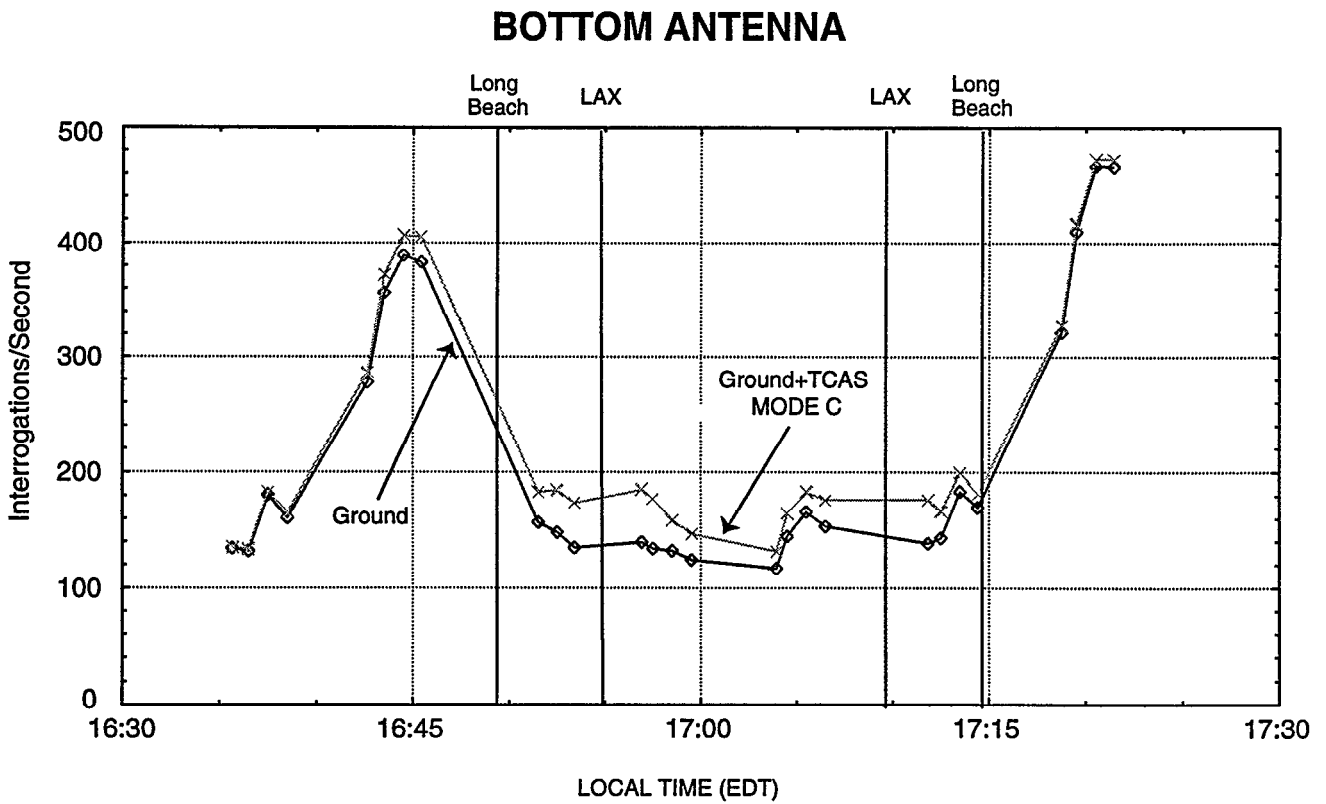
Figure 12. Measured interrogation rates, Los Angeles Basin. The upper curve includes all received ATCRBS interrogations. The lower curve is the subset not including TCAS Mode C interrogations, which are distinguishable by the presence of the P4 pulse [Reference 3]. These results indicate that interrogation rates are high, especially in the vicinity of Long Beach, and that these high rates were transmitted from the ground.
