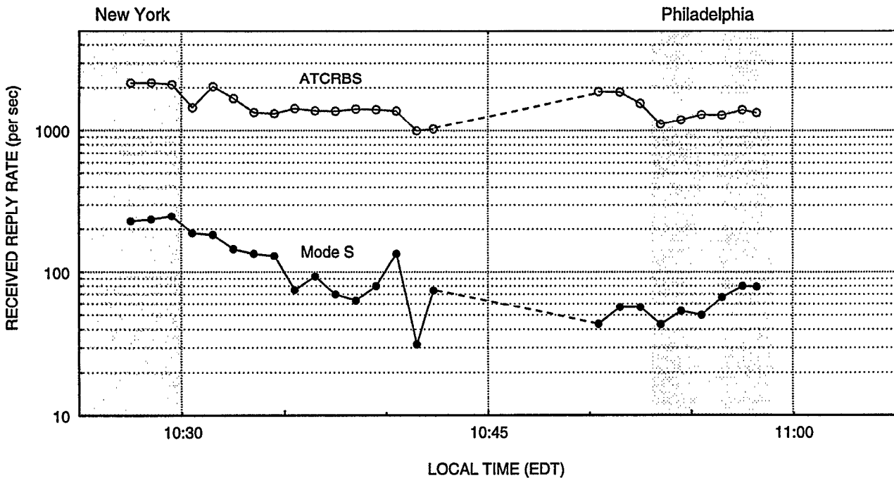
Figure 5. Measured reply rates, New York and Philadelphia. This is the main type of result obtained by airborne AMF recording followed by analysis of the recorded data. Mode S reply rates are lower than ATCRBS reply rates by a large factor. The maximum rates were observed in the New York area.
