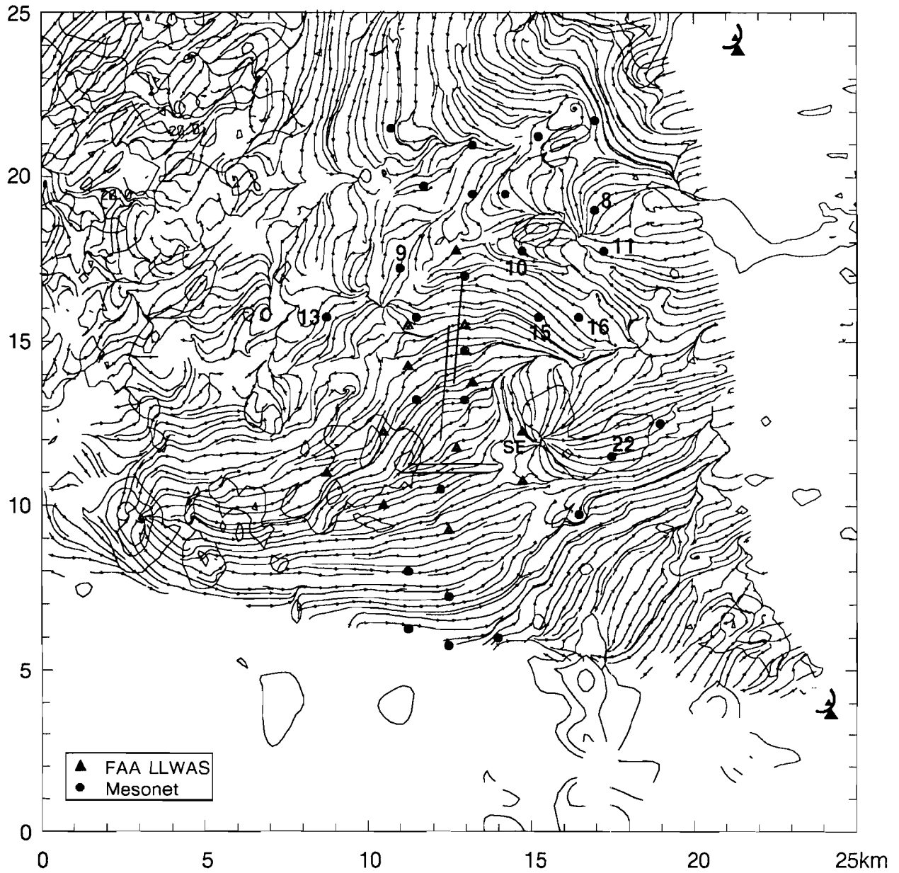
Figure VIII-8b. Dual Doppler plot of the streamline and reflectivity field at 2253:22 UTC on 2 September 1987. This image shows the microbursts more clearly than the wind vector image in Fig. VIII-8a.
