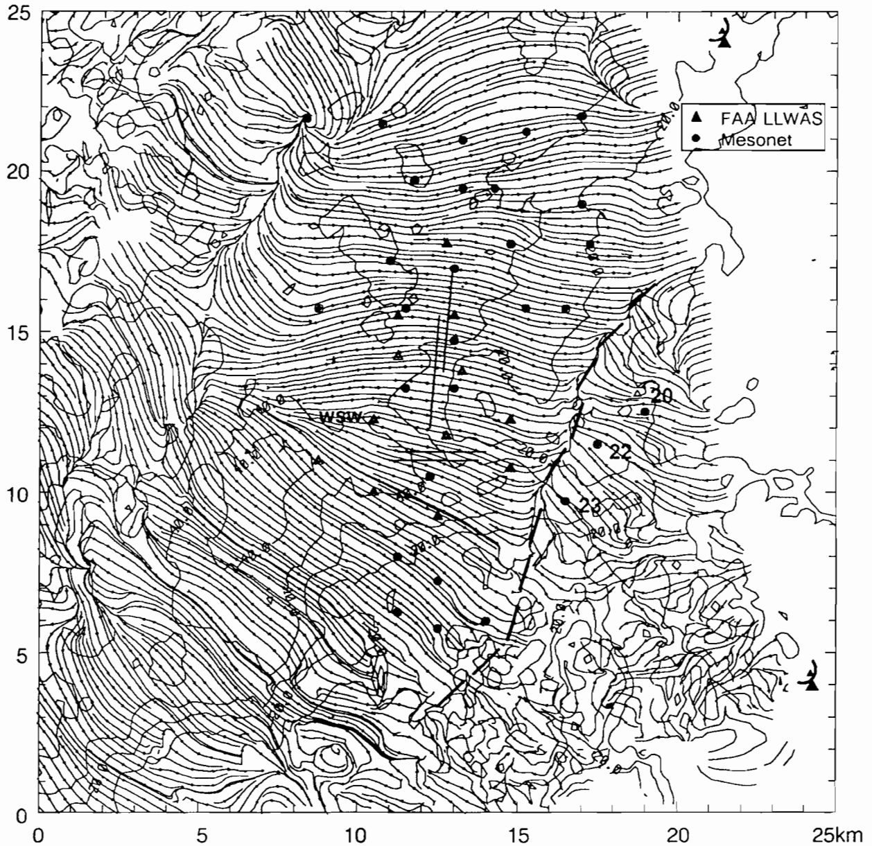
Figure VI-7b. Dual Doppler plot of the streamline and reflectivity field at 0026:14 UTC on 26 August 1987. The MBIdiv line is clearly evident in the northwest quadrant and the dashed line denotes the gust front boundary. Both of these wind shear lines are moving from the northwest toward the southeast.
