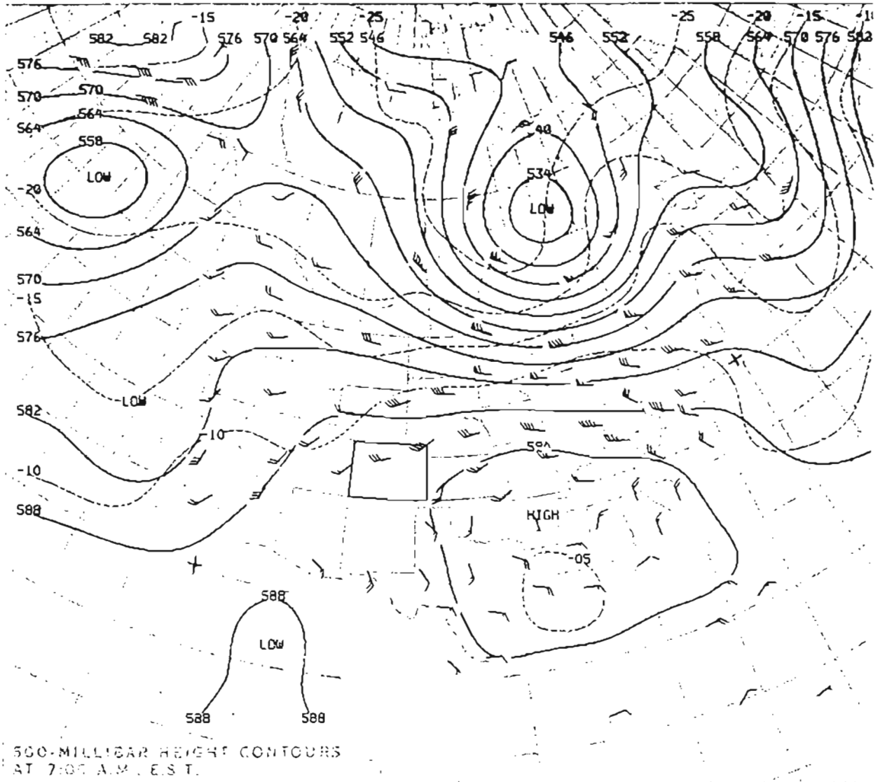
Figure V-2. 500 mb heights/winds representing 1200 UTC observations on 22 August 1987. Map represents upper level winds 14 hours after the gust front had moved through Stapleton. A full barb is 10 knots, a half barb is 5 knots, and a blackened triangle denotes 50 knots. Solid contours are geopotential heights of the 500 mb pressure level in decameters; dotted contours are isotherms in degrees Centigrade.
