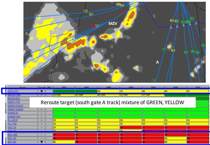
Figure 16. Use of RAPT to plan proactive weather-avoiding reroutes from west gate to south gate.
