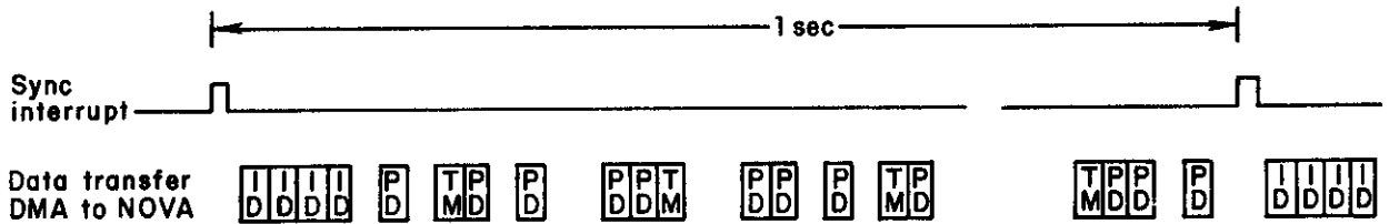
Fig. 9. Typical data stream to NOVA.
