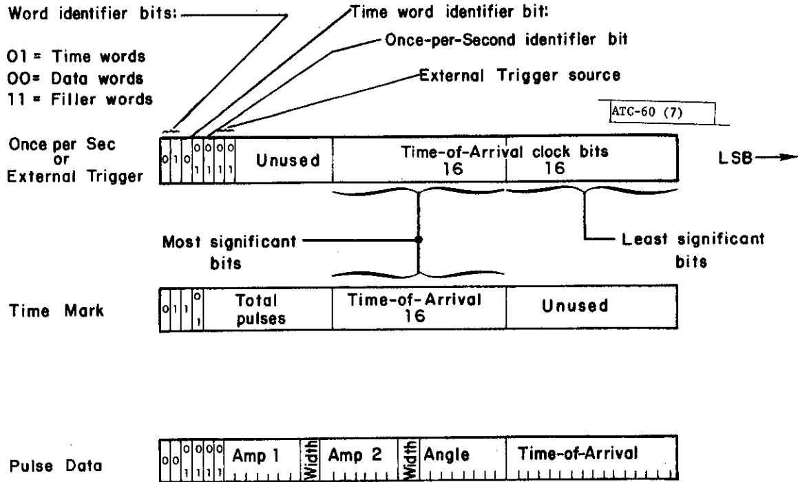
Fig. 7. Time and Data Word formats.
