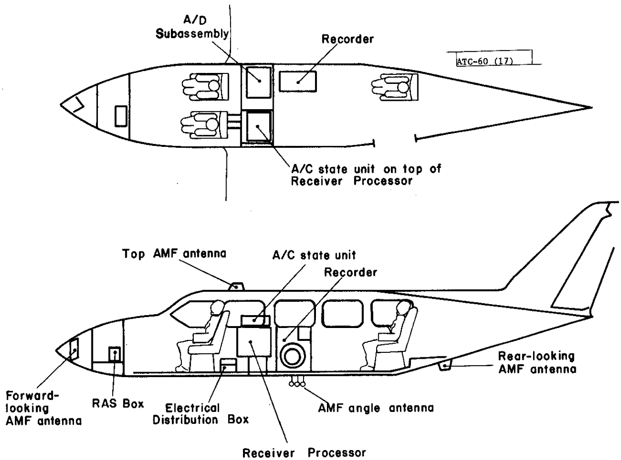
Fig. 17. Typical AMF airborne installation.
