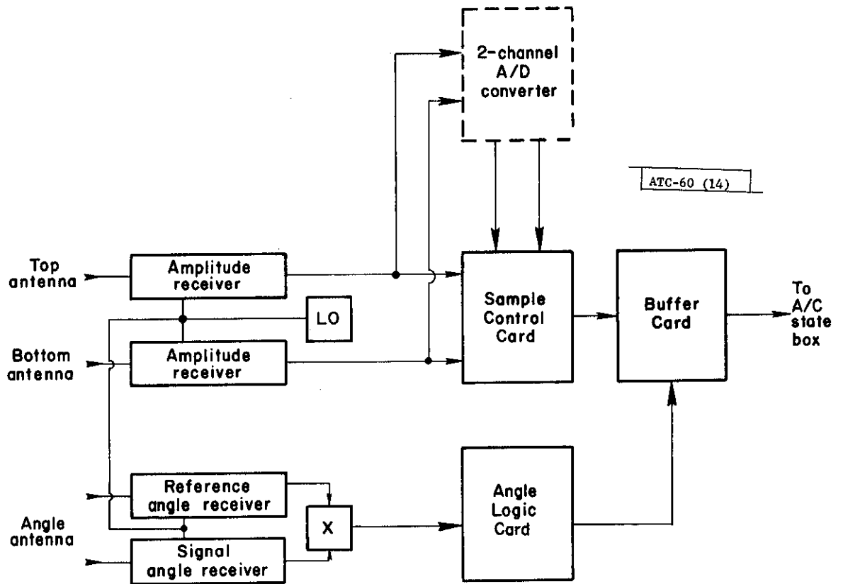
Fig. 14. Receiver-processor unit block diagram.
