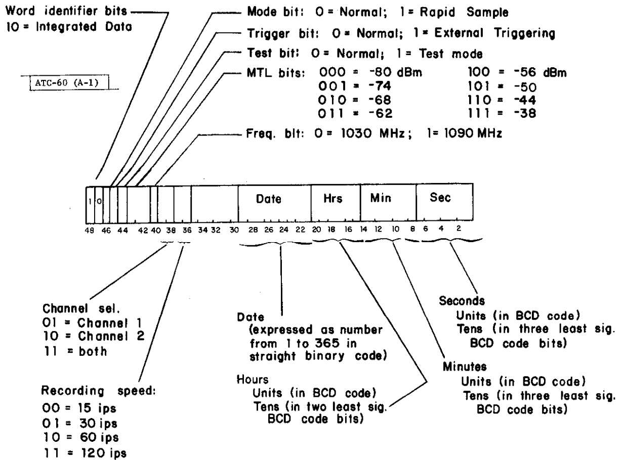
Fig. A-1. Integrated Data Word 1.
