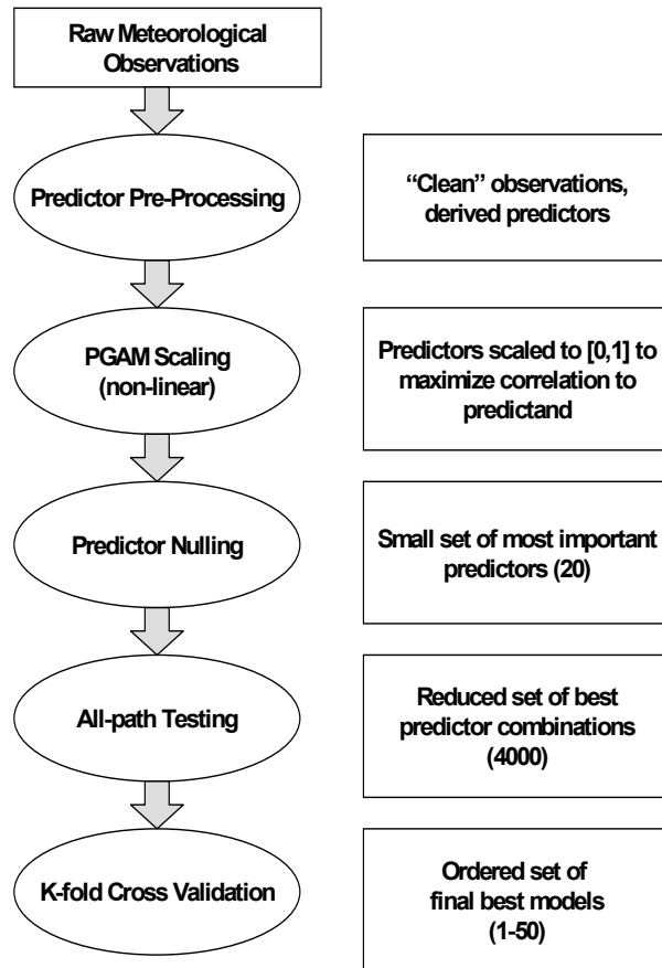
Figure A-1. Schematic overview of SFM-building process.
