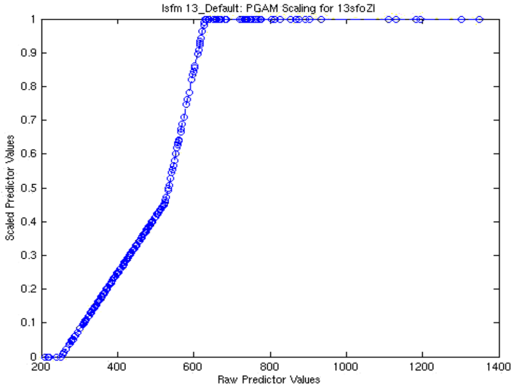
Figure A-2. Piece-wise linear PGAM structure that scales the 13Z SFO inversion height to [0,1]. The structure function can be expressed by the following triplets: (200,0,0), (252,0,0.00167), (525,0.457,.00518), and (630,1,0).
