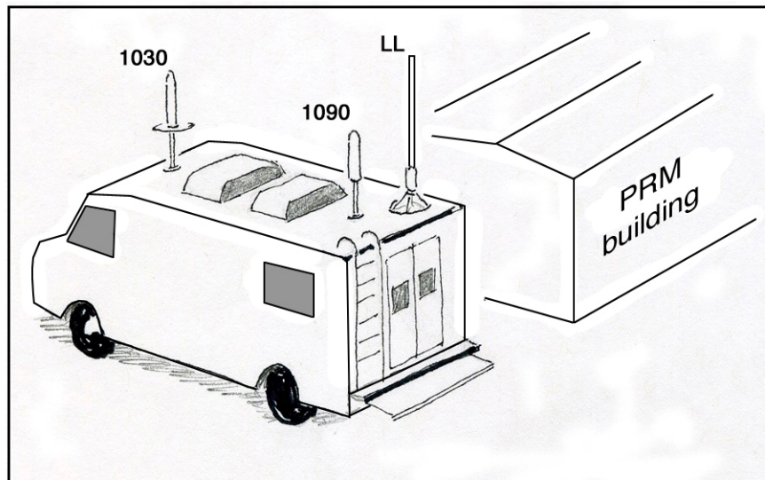
Figure 14. Antenna installation of Philadelphia data collection
