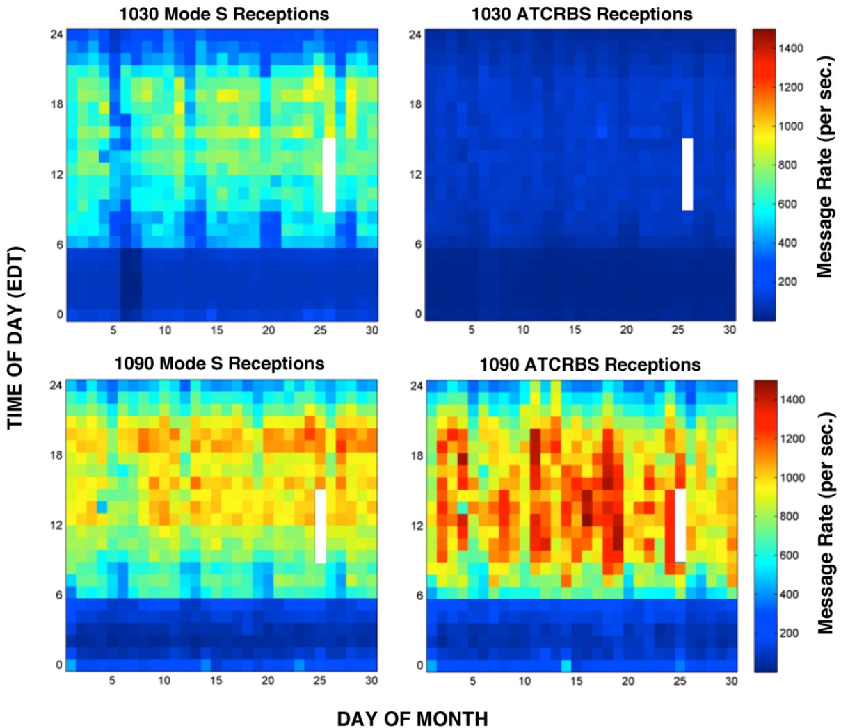
Figure 19. Message reception rate in time (1030 and 1090 MHz) June 2010 Receiver threshold ~ -80 dBm at antenna
