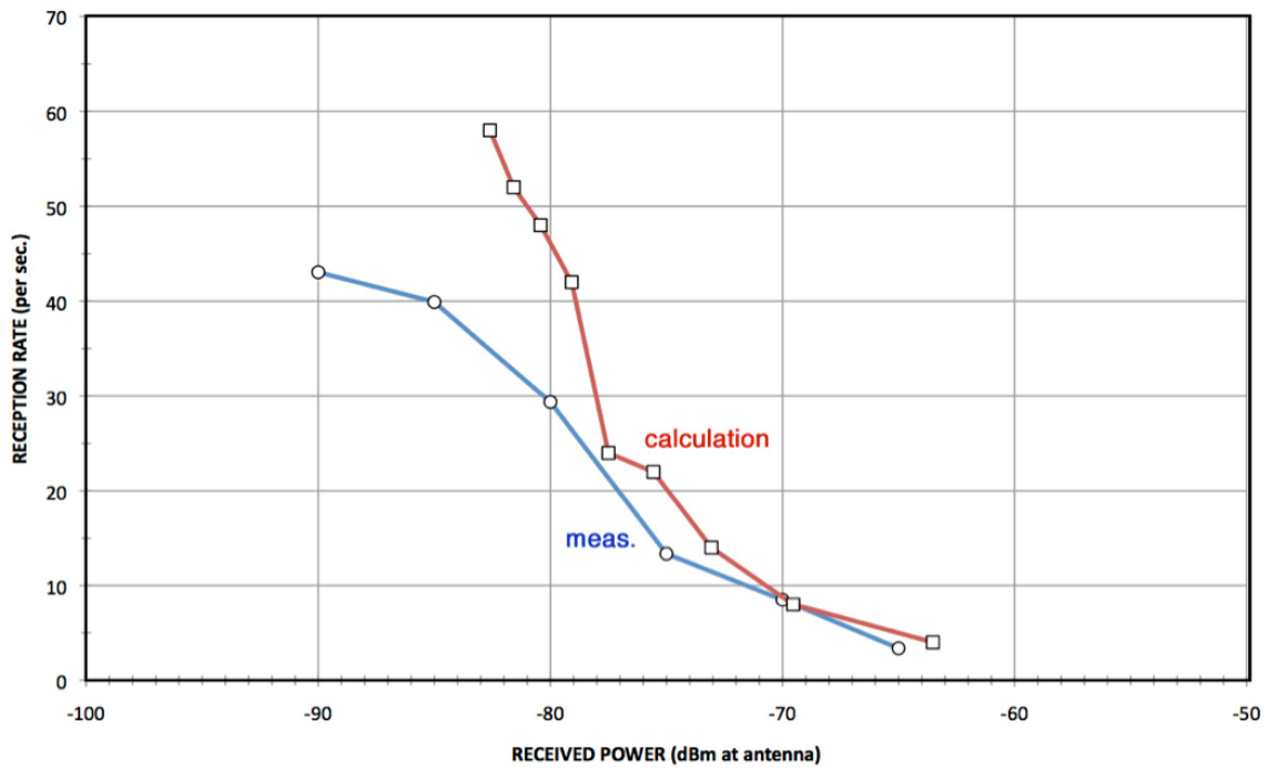
Figure 11. Measurements compared with calculations (Airborne Position Squitters)
