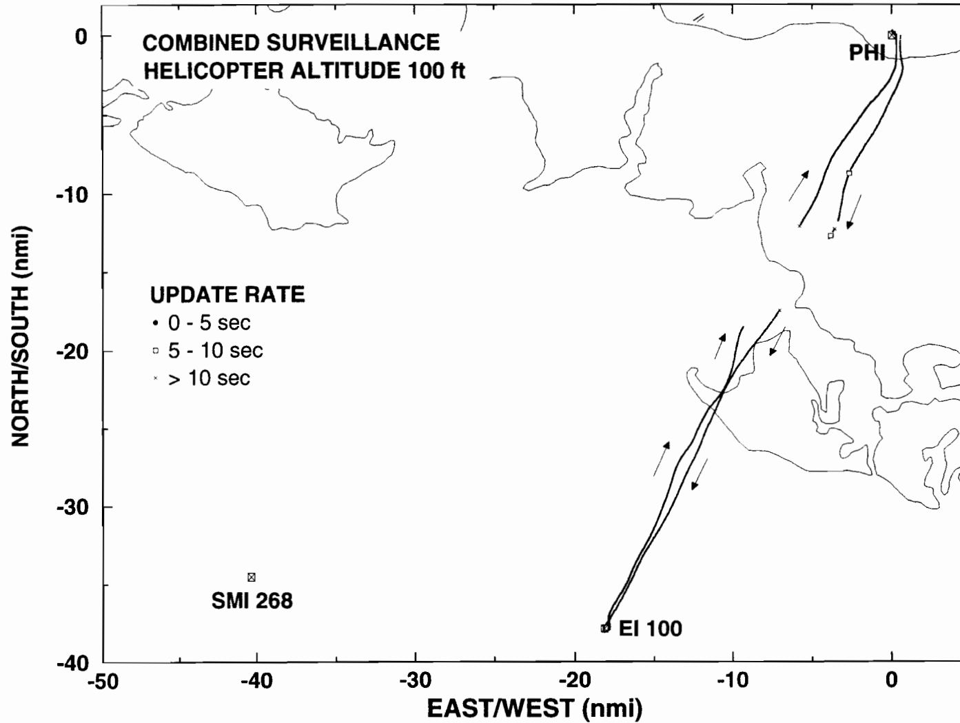
Figure 5-4d. GPS-Squitter surveillance of the Wiggins Bell 206, during a flight to EI 100 at 100-ft altitude, from the three ground stations combined.
