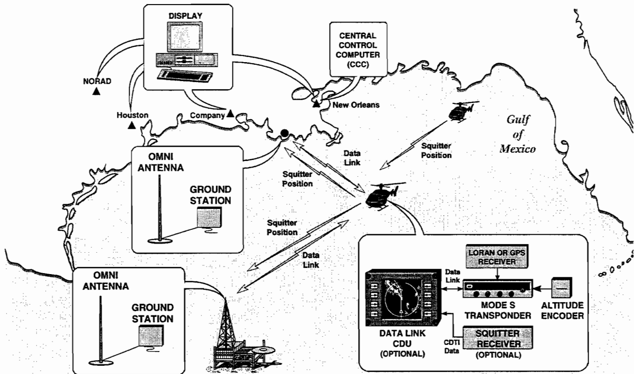
Figure 6-2. Equipment for an offshore region operational system providing both ADS-B surveillance and two-way data link.
