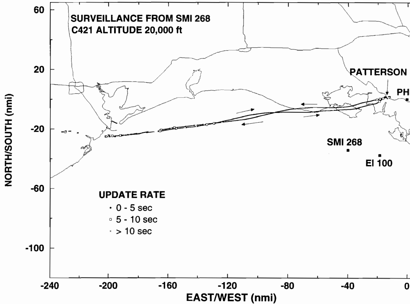
Figure 5-8b. GPS-Squitter surveillance of the Cessna 421, during a long range flight at 20,000-ft altitude, from the ground station at SMI 268.
