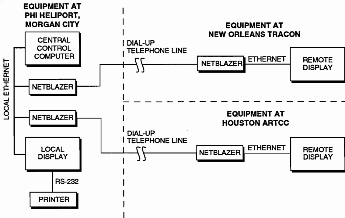
Figure 3-10. Communications from the Central Control Computer to the traffic displays.
