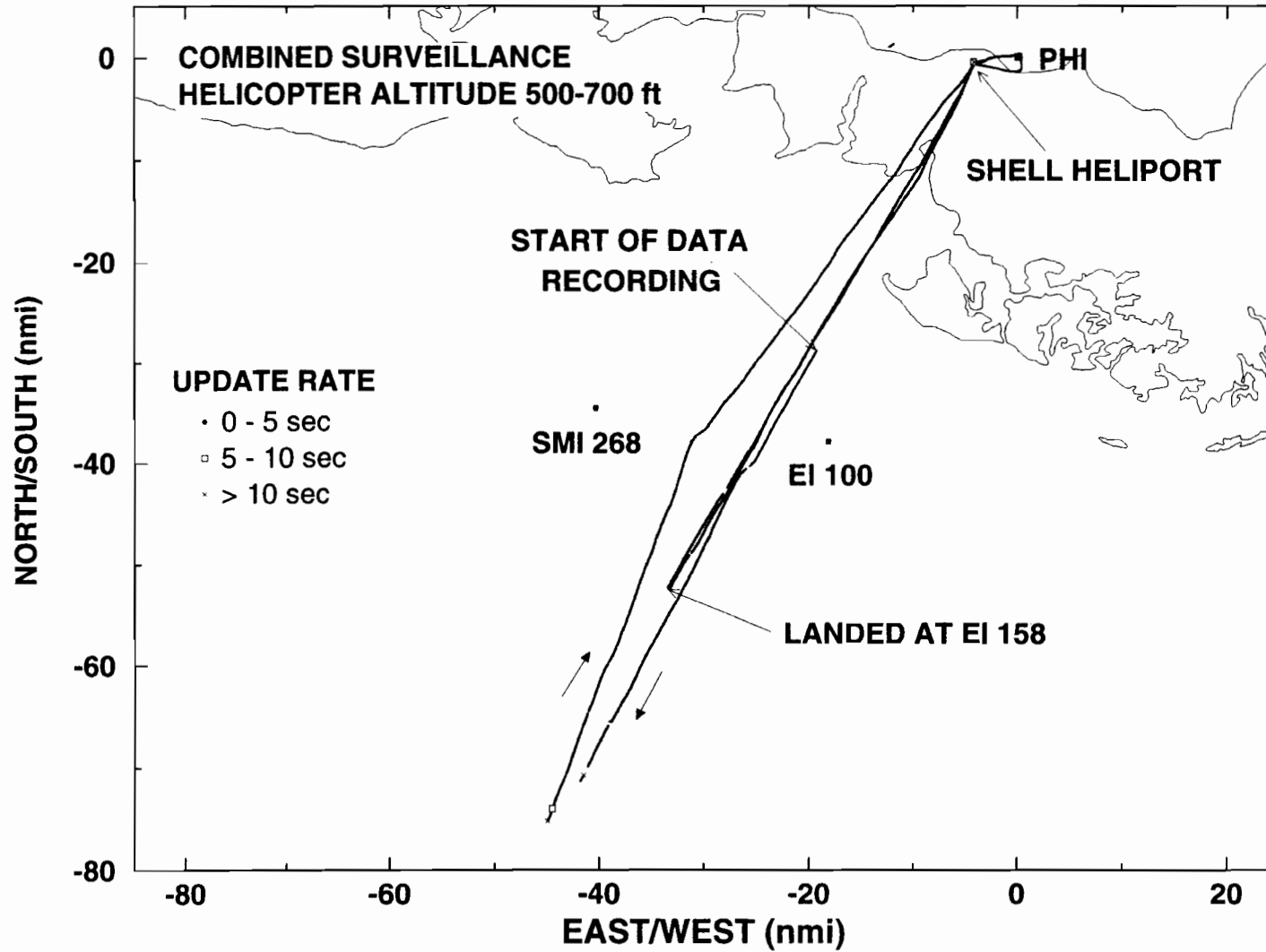
Figure 5-7. Combined GPS-Squitter surveillance of the PHI Bell 206.
