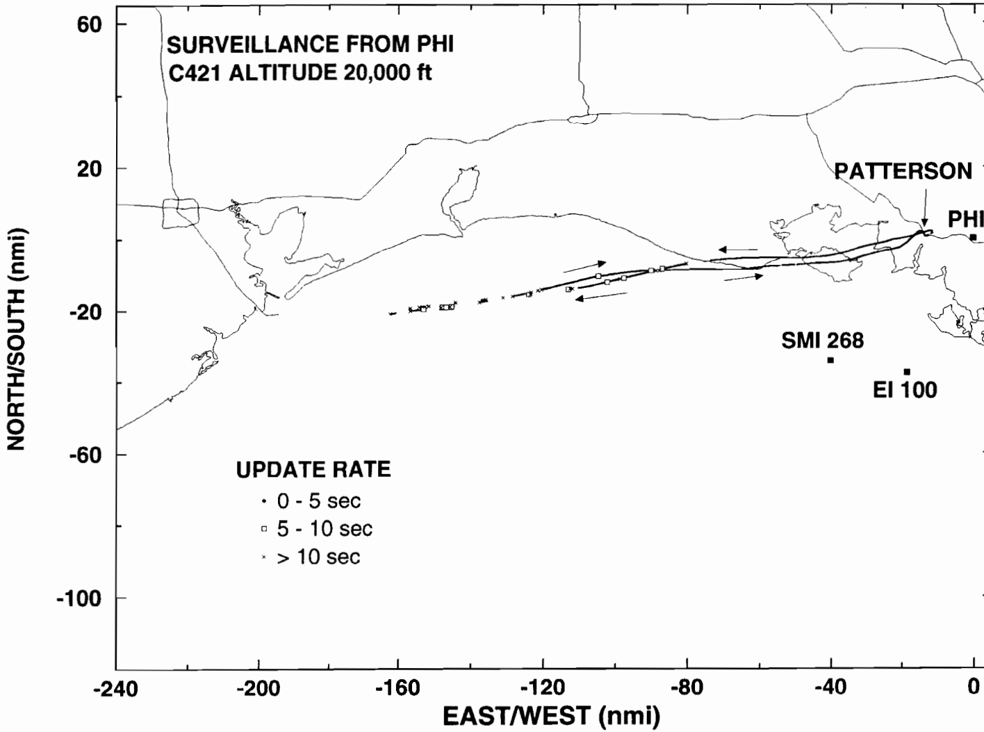
Figure 5-8a. GPS-Squitter surveillance of the Cessna 421, during a long range flight at 20,000-ft altitude, from the ground station at PHI.
