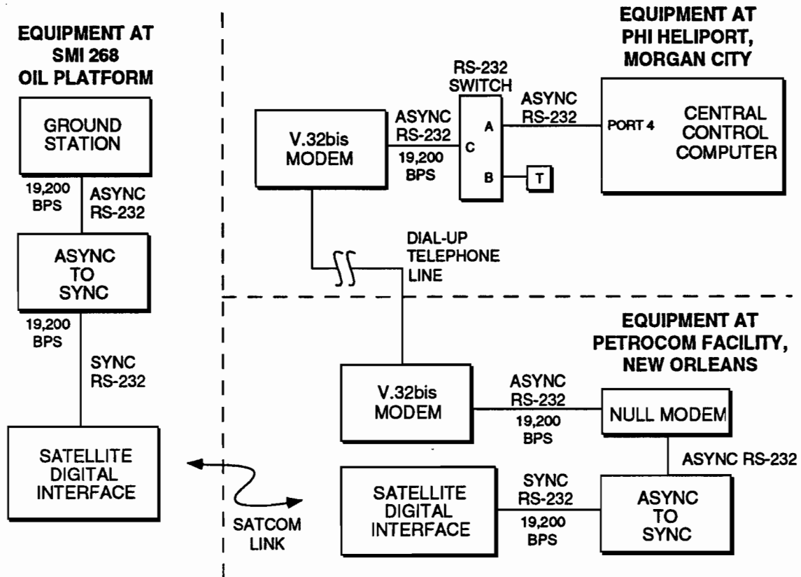
Figure 3-9. Communication link from the SMI 268 ground station to the Central Control Computer.
