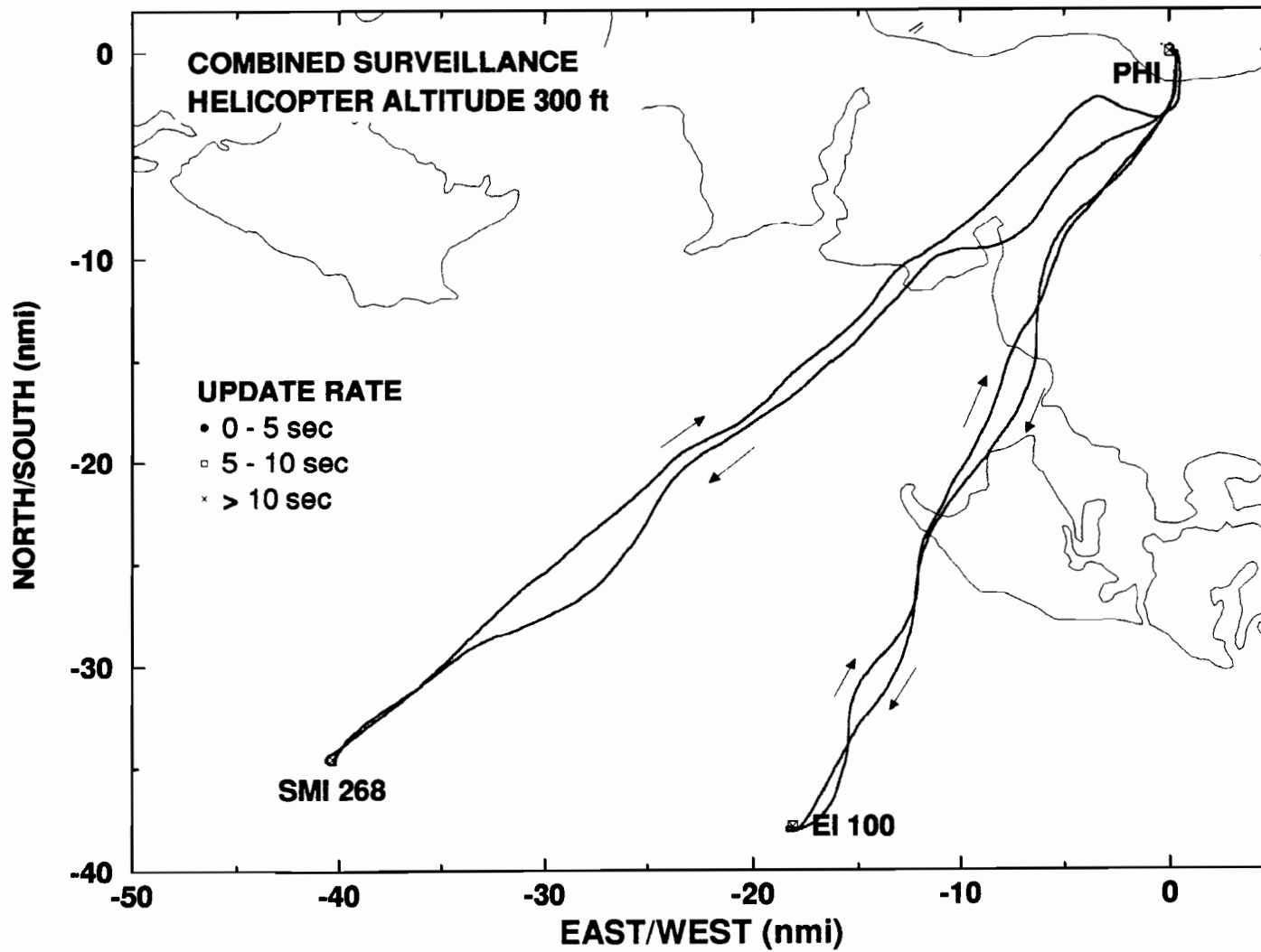
Figure 5-5. Combined GPS-Squitter surveillance of the Wiggins Bell 206 during flights to SMI 268 and EI 100 at 300-ft altitude.
