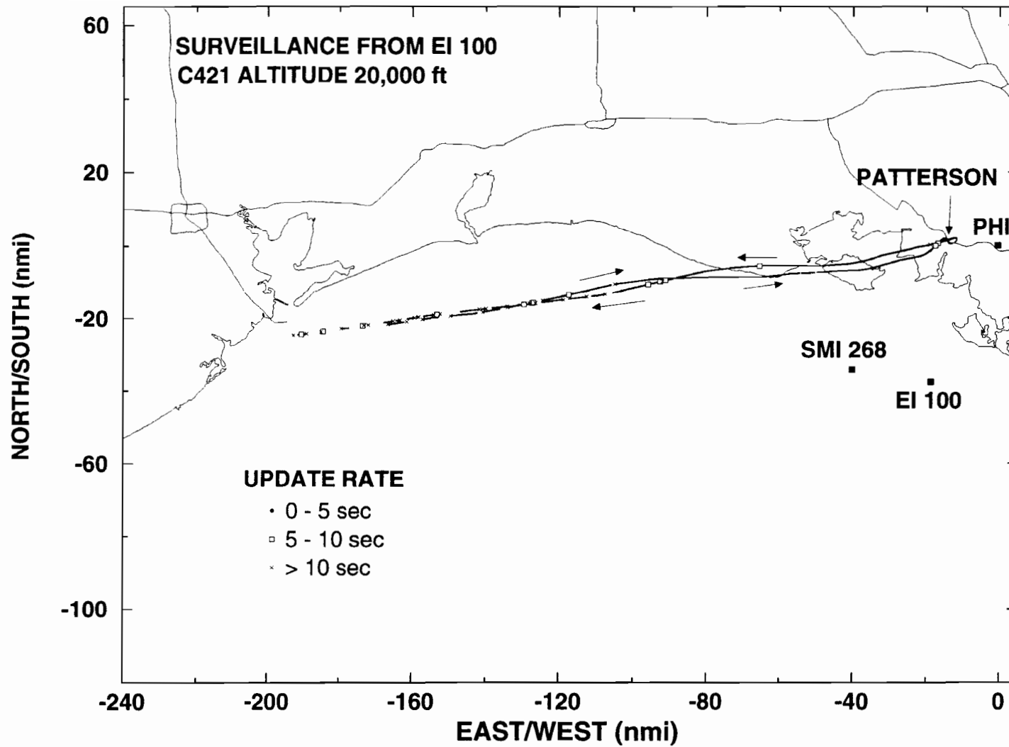
Figure 5-8c. GPS-Squitter surveillance of the Cessna 421, during a long range flight at 20,000-ft altitude, from the ground station at EI 100.
