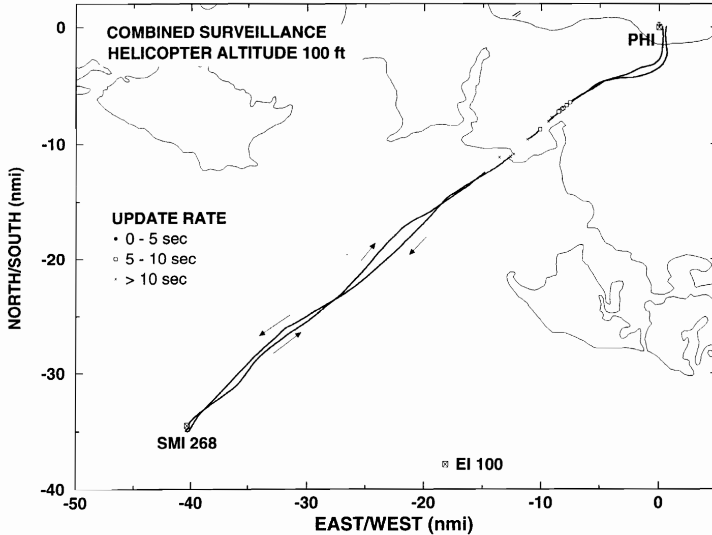
Figure 5-3d. GPS-Squitter surveillance of the Wiggins Bell 206, during a flight to SMI 268 at 100-ft altitude, from the three ground stations combined.
