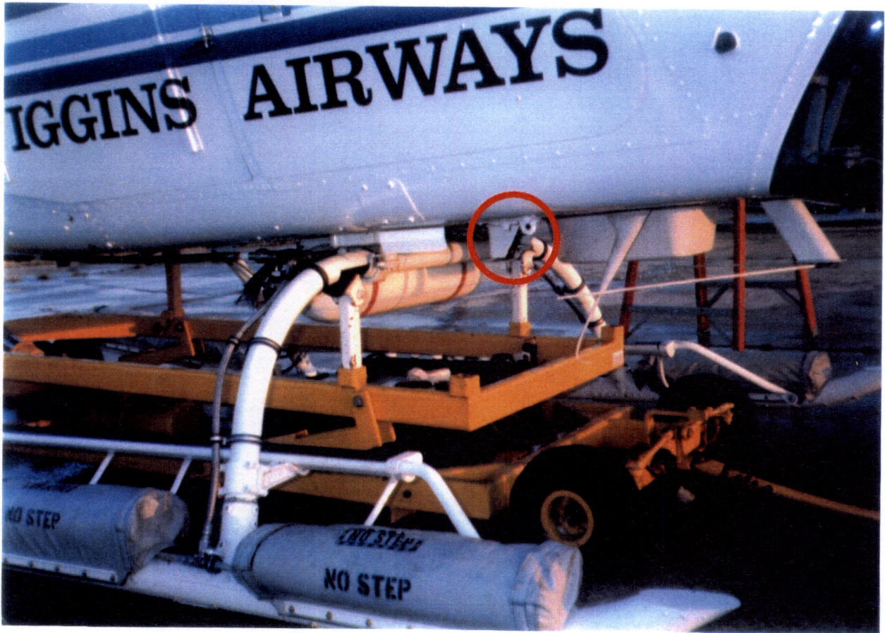
Figure 5-1. Transponder antenna mounted on the underside of the Wiggins Bell 206 helicopter.
