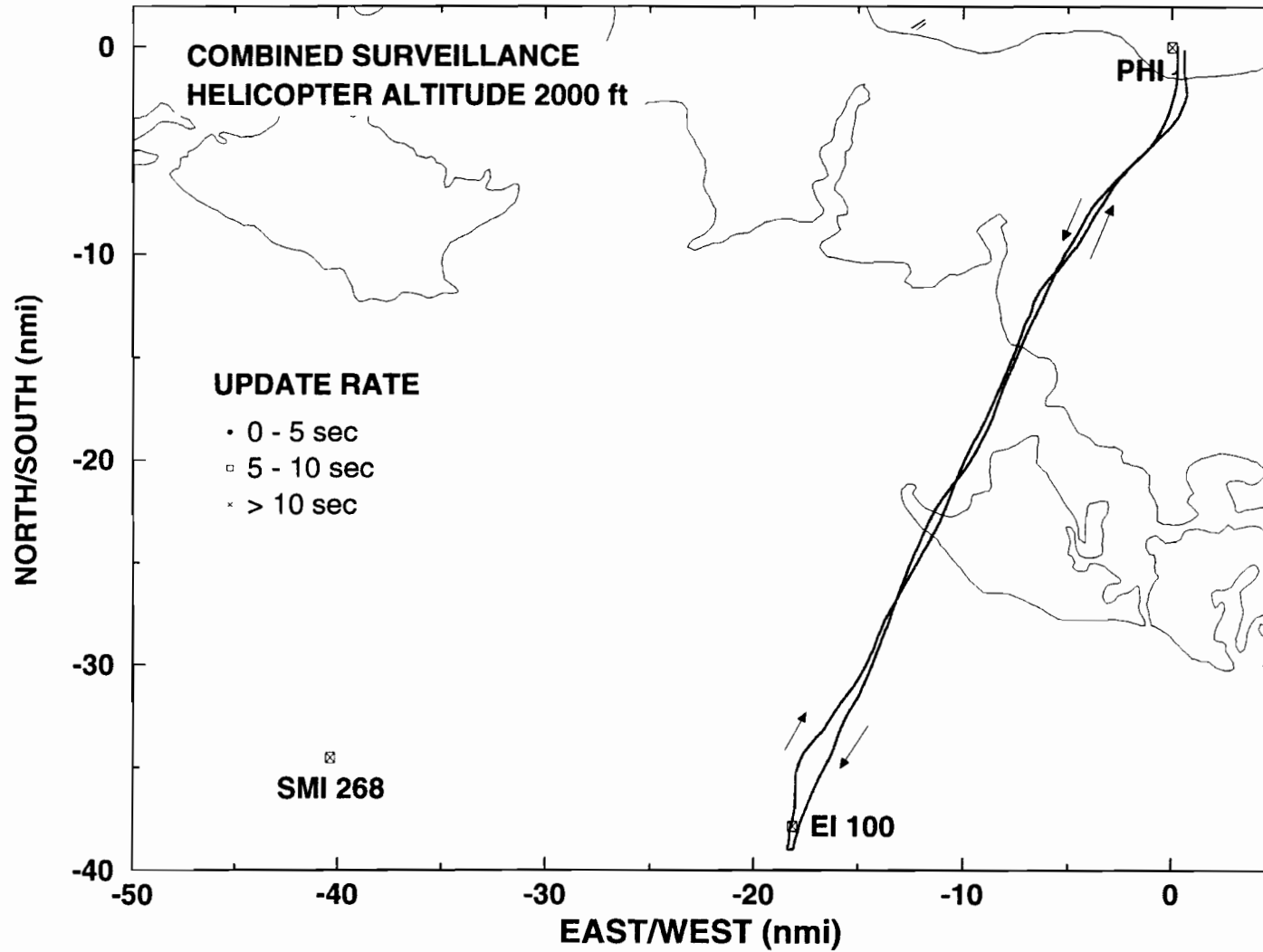
Figure 5-6. Combined GPS-Squitter surveillance of the Wiggins Bell 206 during flights to EI 100 at 2000-ft altitude.
