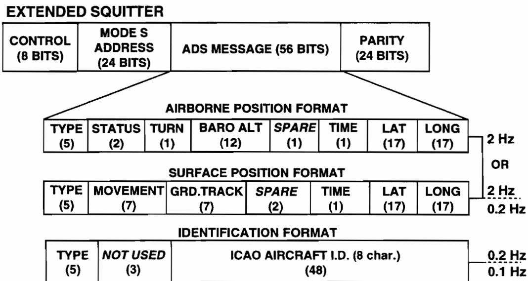
Figure 1-1. Information contained within the three types of extended squitter messages.
